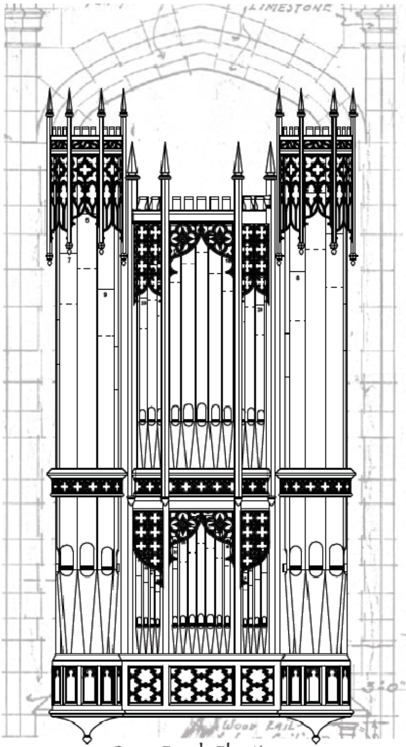
Organ Facade Elevation
