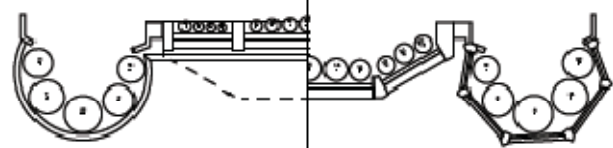
Lower Plan Upper Plan
